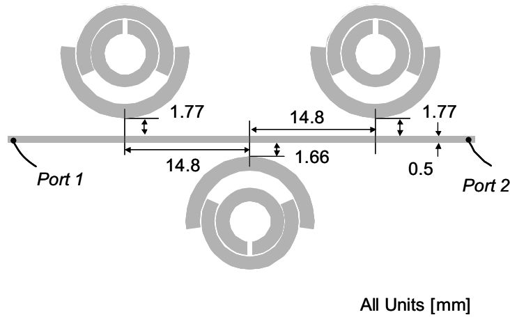
Fig. 4. Structure of reaction-type filter.
