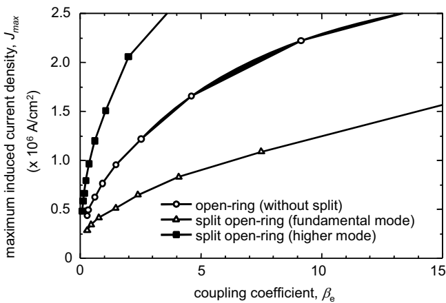
Fig. 2. Resonator coupling coefficients \beta_e against maximum induced current densities.
