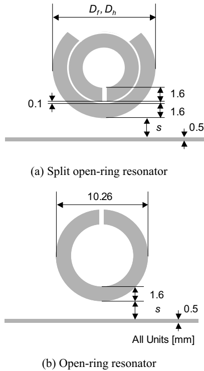
Fig. 1. Structure of the resonators.
