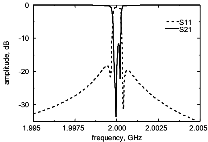
Fig. 5. Frequency characteristics of reaction-type filter.
