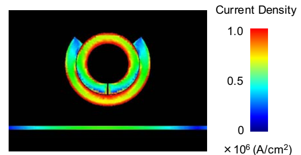
(b) Split open-ring resonator (fundamental mode)
