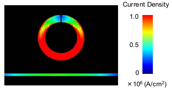
(a) Open-ring resonator
