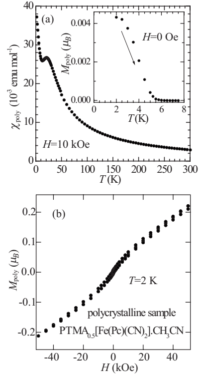
FIG. 4. (a) Temperature dependence of the magnetic susceptibility for bulk polycrystalline samples of \text{PTMA}_{0.5}[\text{Fe}(\text{Pc})(\text{CN})_2] \cdot \text{CH}_3\text{CN} . The inset shows the spontaneous magnetization measured at the zero field. (b) Magnetization at 2 K, as a function of the field for a polycrystalline sample. Note the anomaly around H=0 .
