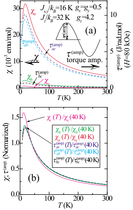
FIG. 6. (Color online) The calculations of the magnetic susceptibilities and magnetic torques. The parameters used in these calculations are g_x = g_y = 0.5 , g_z = 4.2 , J_x = J_y = 16 K, and J_z = 32 K. These were the same parameters used for the calculation of the magnetic properties of TPP[Fe(Pc)(CN) 2 ] 2 . (See Ref. 12.) (a) The temperature dependence of the magnetic susceptibilities for the field applied to the crystallographic a , b , and c axes ( \chi_a, \chi_b, \chi_c ) and the magnetic torque amplitude for the field rotated within the ab , bc , and ac plane [ \tau_{ab}^{(amp)} , \tau_{bc}^{(amp)} , and \tau_{ac}^{(amp)} ]. (b) Temperature dependence of these values normalized by the values at 40 K.
