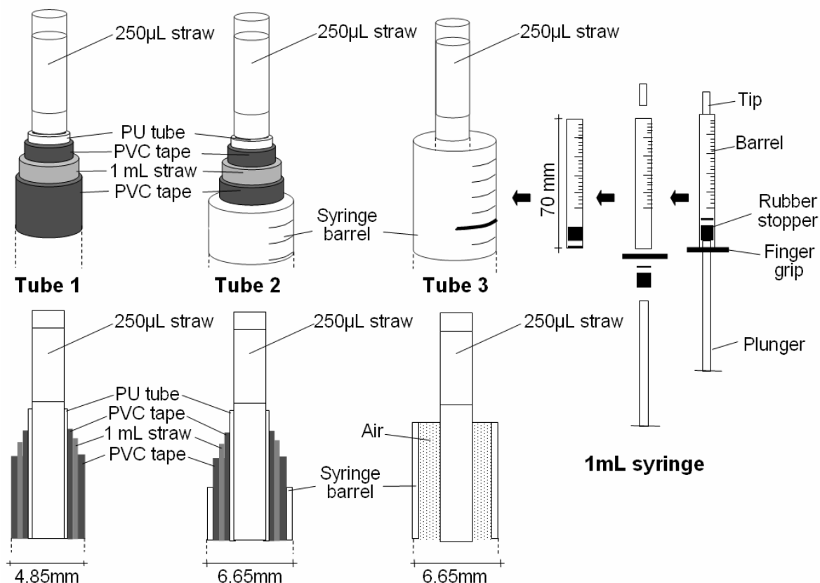
Figure 1. Structure and longitudinal section (lower) of the three different tubes used to control cooling rates for cryopreservation. Details of materials are the following: polyurethane tube (PU) - internal diameter: 2.04mm, external diameter: 3.23mm (Argyle, Japan); 1mL straw tube - internal diameter 3.91mm, external diameter 4.18mm (IMV, France); 1mL syringe tube - internal diameter: 4.66mm, external diameter: 6.6mm (Terumo, Japan) and polyvinyl adhesive tape (PVC). Schematic representation for preparation of tube 3 using 1mL syringe is detailed (right). Tip and finger grip are detached from the barrel and discharged. Rubber stopper is detached from the plunger, inverted and placed in the barrel extreme. A 250µL straw was cut to adequate to the barrel length (70mm) resulting in a 130µL final volume. All the tubes had the same length (70mm).
