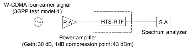
Fig. 9 The schematic diagram of the ACLR estimation using W-CDMA four-carrier signal.
