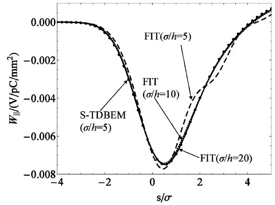
Fig. 8. Longitudinal dipole wake potential calculated with a simple 2.5-D FIT scheme with square mesh and 2.5-D S-TDBEM scheme for the TESLA 9cell cavity excited by a Gaussian bunch with \sigma = 5 mm and with an offset a = 1 mm to the axis.
