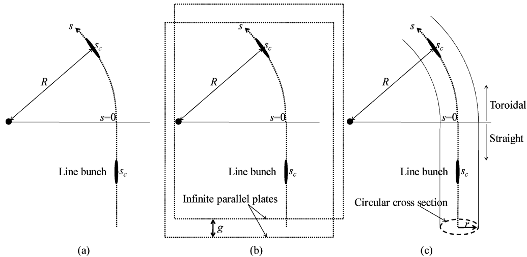
Fig. 11. Vacuum chamber geometries tested for transient analysis of wake fields generated by a Gaussian line bunch moving with curved trajectory. (a) Free space model, (b) infinite parallel plate model, (c) pipe-like vacuum chamber with circular cross section.
