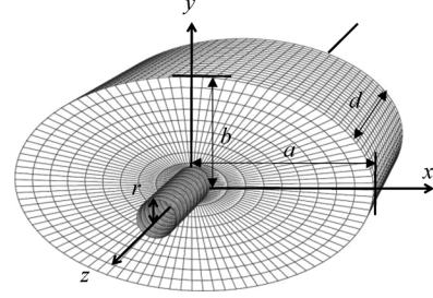
Fig. 4. Numerical model of elliptical pillbox cavity with small beam pipes.
