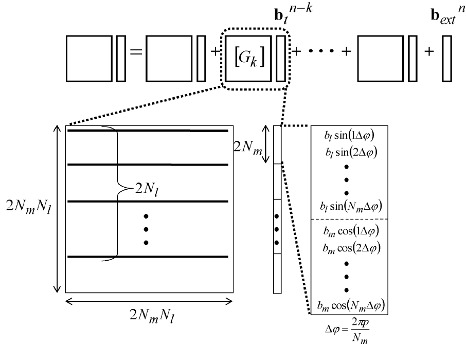
Fig. 2. The sin / cos dependencies of boundary value vector in A3D S-TDBEM system matrix equation for azimuthal mode p . In the A3D scheme, one needs to store only first row among the boundary elements with same radius [8]–[10], and therefore matrix size becomes 2N_l \times 2N_l N_m without taking into account the sparseness of the matrix. However, in a time domain simulation the amount of overall operation is almost same as that of the full 3-D scheme since all boundary values over a 2-D surface have to be solved.
