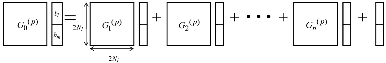
Fig. 3. Structure of the reduced 2.5-D TDBEM matrix equation for azimuthal mode m .
