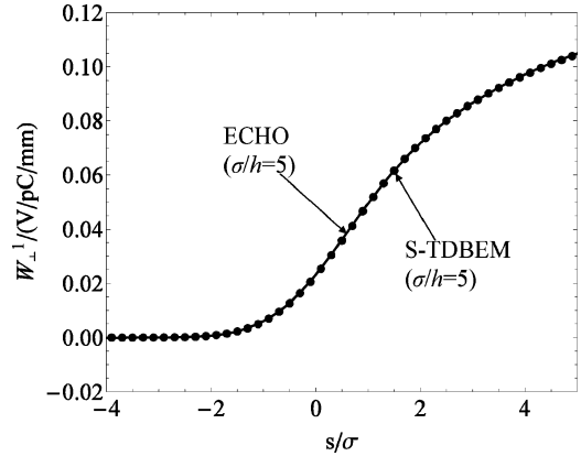
Fig. 9. Comparison of transverse dipole wake potentials calculated by different dispersion-free codes for the TESLA 9cell cavity excited by a Gaussian bunch with \sigma = 2 mm and with an offset ( a = 1 mm) to the axis. The both calculations are done with a coarse mesh resolution ( \sigma/h = 5 ).
