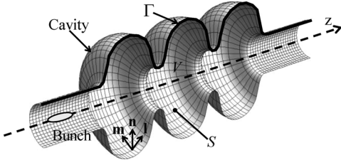
Fig. 1. Typical example of wake field analysis: a charged particle bunch traversing an axially symmetric accelerating cavity.
