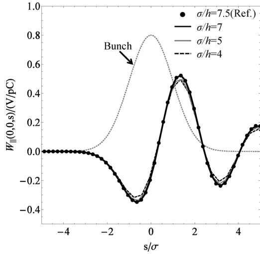
Fig. 6. Convergence of longitudinal wake potential of the elliptical pillbox cavity calculated with the full 3-D S-TDBEM code.
