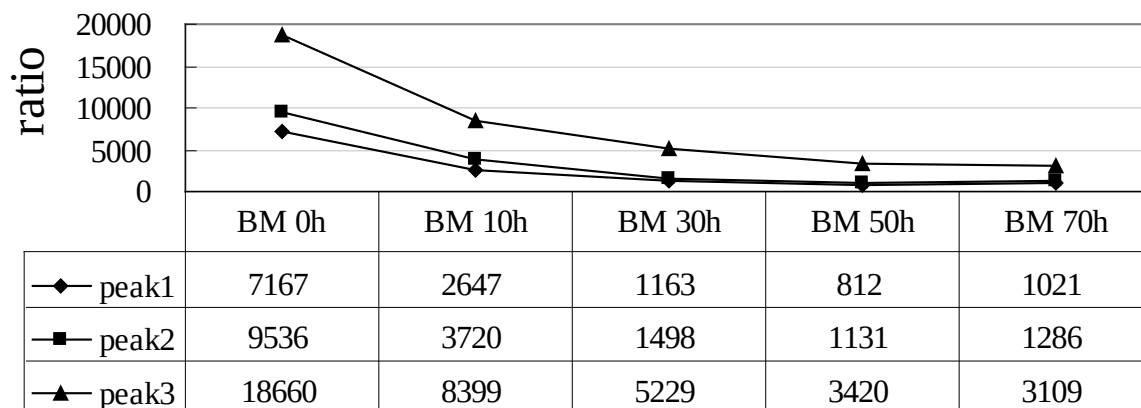
Figure 6 XRD peaks data of the combustion-synthesized products by using different ball-milling time.
