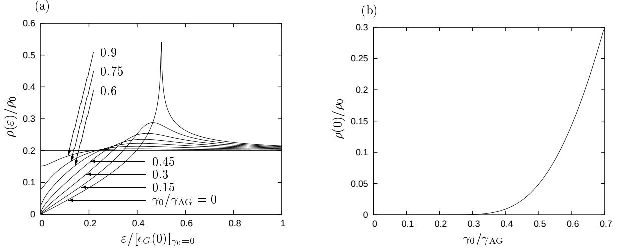
FIG. 5: (a) Density of states \rho(\epsilon) for \gamma_0/\gamma_{AG} = 0, 0.15, 0.3, 0.45, 0.6, 0.75 , and 0.9 and (b) \rho(\epsilon = 0) at T = 0 K as a function of \gamma_0/\gamma_{AG} . In the model of this paper, \rho(\epsilon) is an even function of \epsilon .
