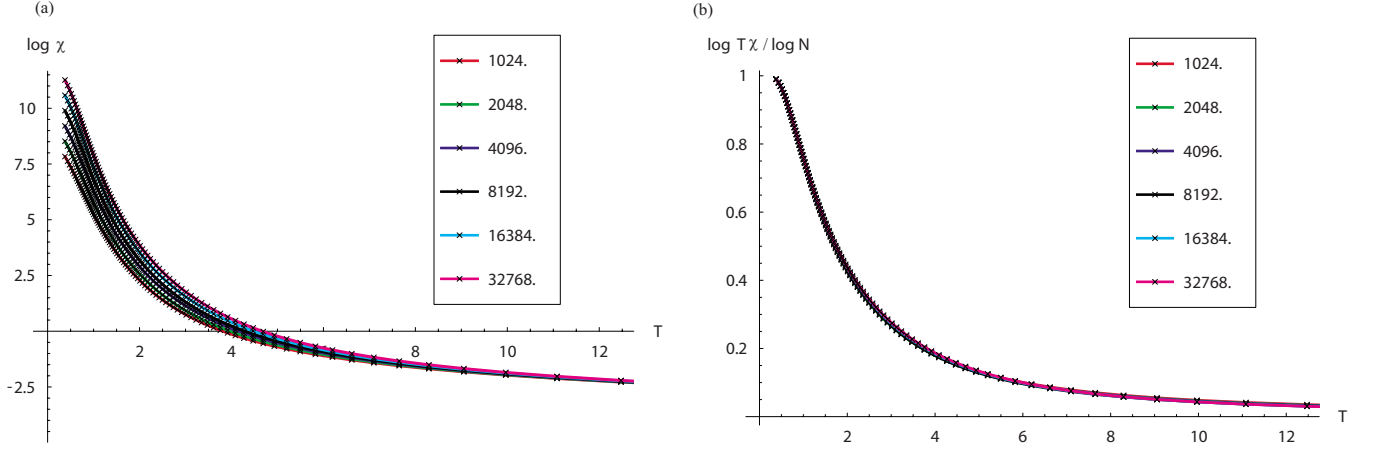
FIG. 4. (Color online) (a) The system susceptibility \ln \overline{\chi_{\text{sys}}} and (b) \ln(T\overline{\chi_{\text{sys}}})/\ln N on the GR tree for no offset \alpha=0 . The number of nodes is taken from N=2^{10} to 2^{15} . The results are averaged over 100 samples.
