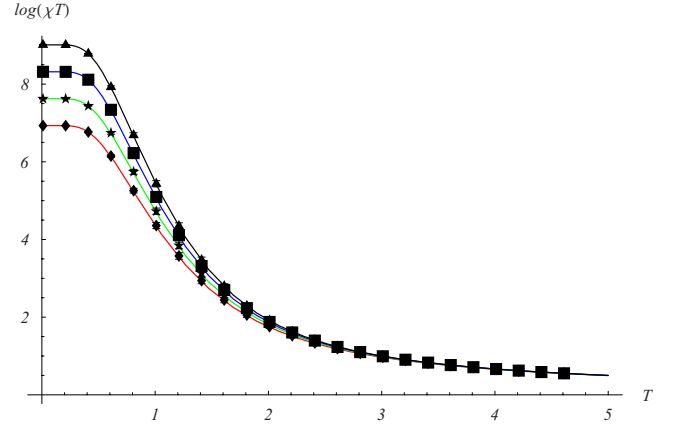
FIG. 1. (Color online) The system susceptibility for the infinite offset by the analytical results [Eq. (10)] (lines) and the numerical ones (points). The numbers of nodes are taken N = 2^{10} (red), 2^{11} (green), 2^{12} (blue), and 2^{13} (black), from bottom to top. The average is taken over 100 samples.
