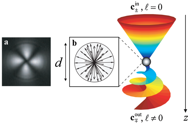
FIG. 1 (color online). Optical vortex generation from a radial nematic liquid crystal droplet. An incident light with circular polarization \mathbf{c}_\pm having a smooth wave front profile ( \ell = 0 ) is partly converted into the orthogonal polarization state \mathbf{c}_\mp that bears a phase singularity ( \ell \neq 0 ). Insets: (a) crossed polarizers image identifying a cylindrically symmetric director distribution and (b) radial structure of the director.
