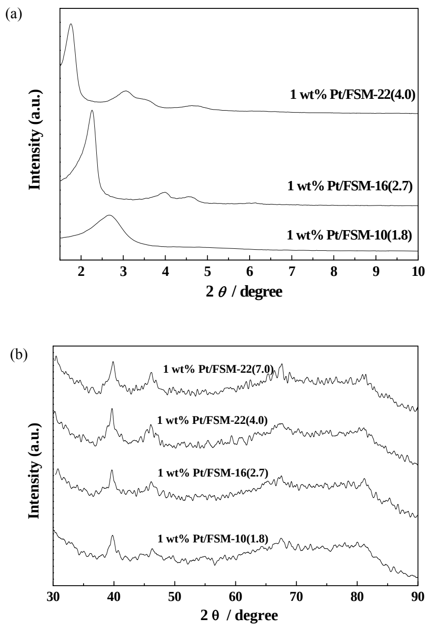
Fig. 1. The XRD patterns of 1 wt% Pt/FSM- n(x) catalysts at low 2\theta angles (a) and at high 2\theta angles (b).
