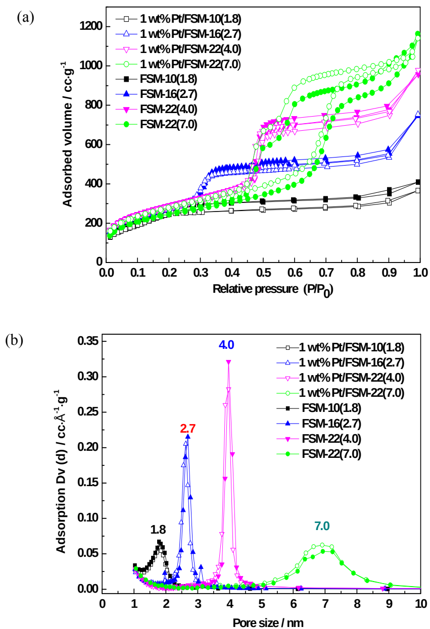
Fig. 2. N 2 adsorption isotherms (a) and pore size distribution curves of FSM- n(x) supports and 1 wt% Pt/FSM- n(x) catalysts (b).
