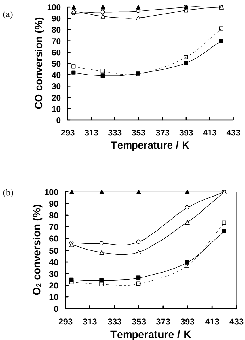
Fig. 4. PROX reaction by 1 wt% Pt/FSM- n(x) under the excess O 2 /CO ratio of 1. (a) CO conversion; (b) O 2 conversion. (■: 1 wt% Pt/FSM-10(1.8), ○: 1 wt% Pt/FSM-16(2.7), ▲: 1 wt% Pt/FSM-22(4.0), △: 1 wt% Pt/FSM-22(7.0), -□--: 1 wt% Pt/SiO 2 ). Conditions: catalyst 0.2 g, CO 1 vol%, O 2 1 vol%, N 2 5 vol%, H 2 balance, space velocity 12000 mLg -1 h -1 , 0.1 MPa.
