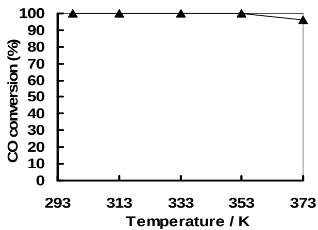
Fig. 6. PROX reaction by 0.5 wt% Pt/FSM-22(4.0) under the stoichiometric O 2 /CO ratio of 1/2. Reaction conditions: catalyst 0.4 g, CO 1 vol%, O 2 0.5 vol%, N 2 5 vol%, H 2 balance, space velocity 3000 mLg -1 h -1 , 0.1 MPa.
