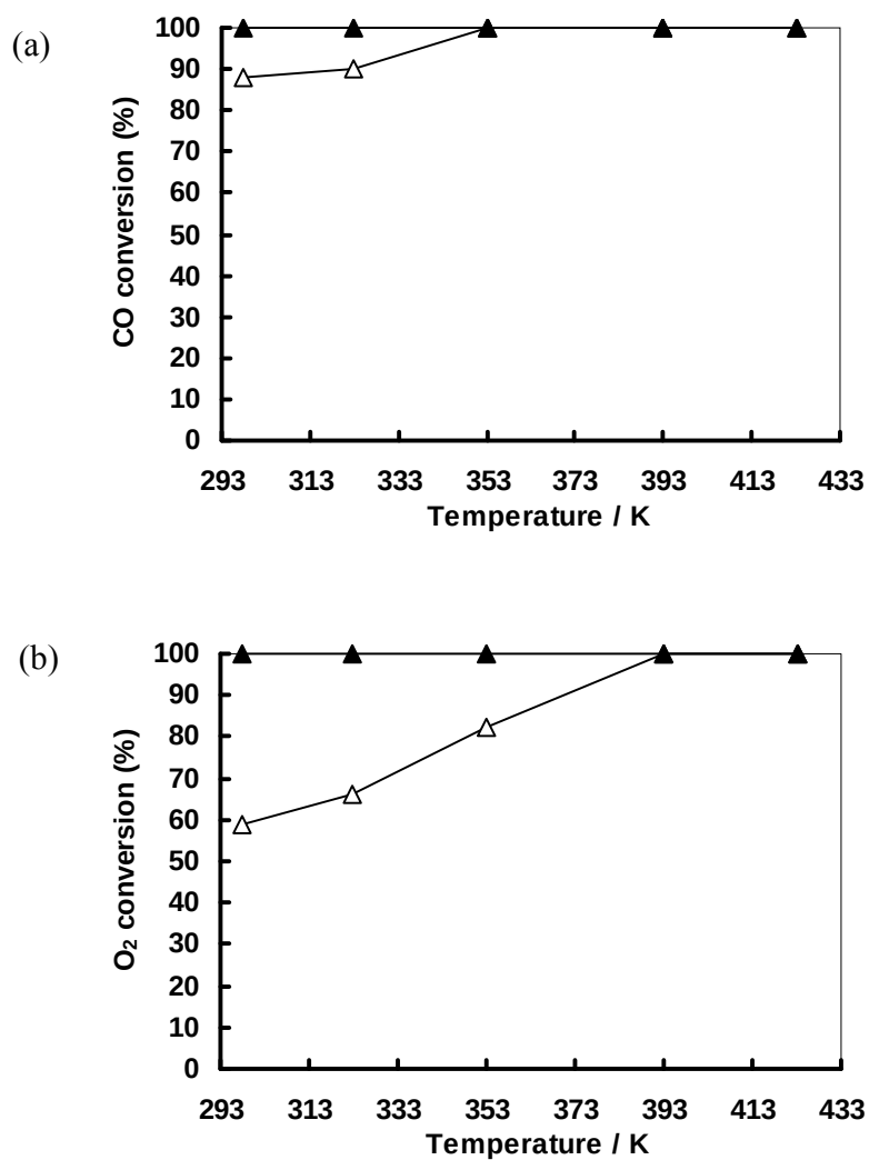
Fig. 5. Catalytic performance of 0.5 wt% Pt/FSM-22(4.0) and 0.5 wt% Pt/FSM-16(2.7). (a) CO conversion; (b) O 2 conversion. (-▲-: 0.5 wt% Pt/FSM-22(4.0);-Δ-: 0.5 wt% Pt/FSM-16(2.7)). Conditions: catalyst 0.4 g, CO 1 vol%, O 2 1 vol%, N 2 5 vol%, H 2 balance, space velocity 3 000 mL g -1 h -1 , 0.1 MPa.
