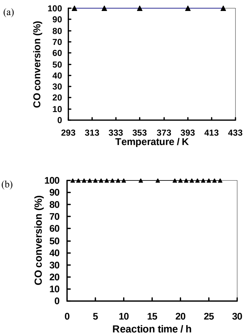
Fig. 7. PROX reaction by 0.5 wt% Pt/FSM-22(4.0) in the presence of water vapor and CO 2 . (a) Reaction conditions: catalyst 0.4 g, CO 1 vol%, O 2 1 vol%, N 2 5 vol%, CO 2 15 vol%, H 2 O 0.9 vol%, H 2 balance, space velocity 3000 mL g -1 h -1 , 0.1 MPa; (b) Reaction conditions: catalyst 0.4 g, CO 1 vol%, O 2 1 vol%, N 2 5 vol%, CO 2 15 vol%, H 2 O 2 vol%, H 2 balance, space velocity 3000 mLg -1 h -1 , 0.1 MPa.
