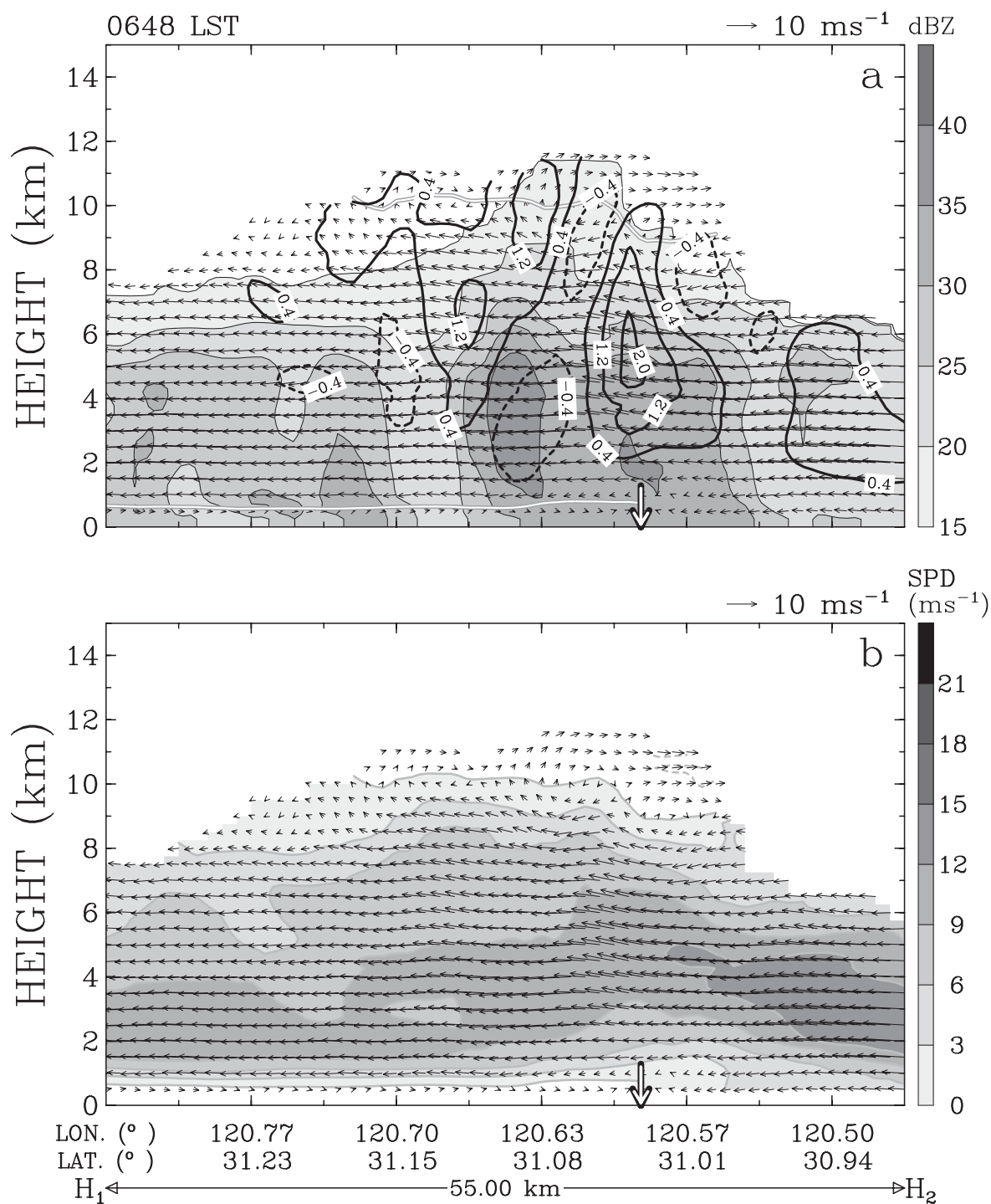
Fig. 19. (a) Vertical cross section of radar reflectivity (shaded), winds along the section plane (arrows), and vertical velocity (contoured every 0.8 \text{ m s}^{-1} ) for 0648 LST 21 June 2002. The section is along line H_1H_2 in Fig. 17. White solid lines represent interfaces of the positive and negative velocities of horizontal winds along the section plane. The approximate location of the front at the surface is indicated by the white vertical arrow. (b) Same as (a) except for the velocity of the horizontal wind component along the section plane (contoured every 3 \text{ m s}^{-1} and shaded above 0 \text{ m s}^{-1} ).
