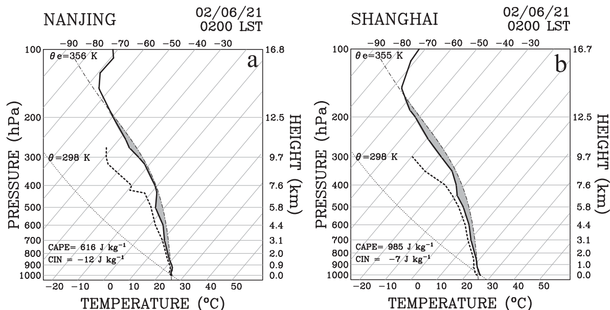
Fig. 4. Skew-T log p diagrams of temperature (bold solid line) and dew point temperature (bold dashed line) at 0200 LST 21 June 2002 from soundings at (a) Nanjing and (b) Shanghai. The shaded region in each figure indicates the positive area (CAPE).
