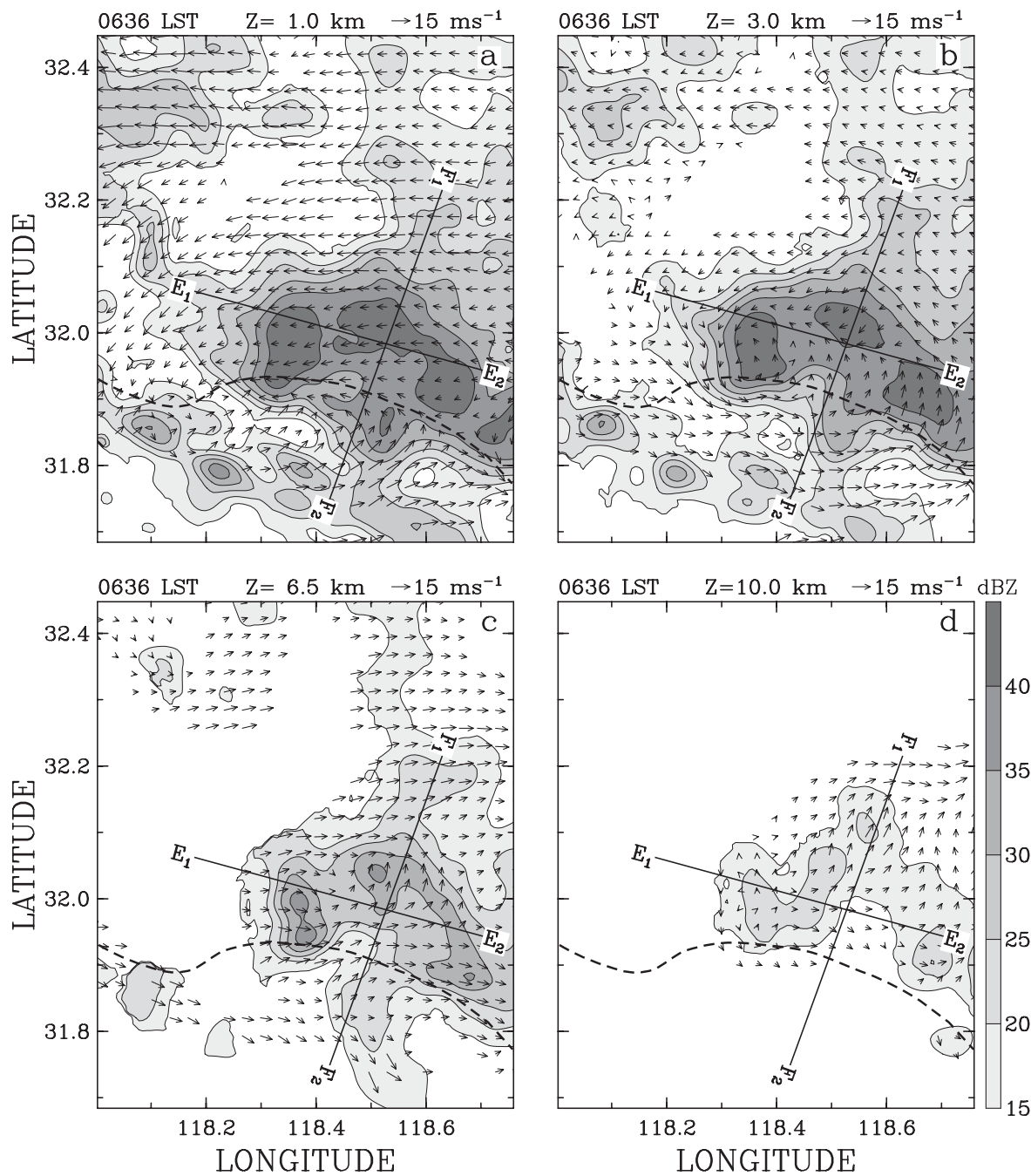
Fig. 14. Same as Fig. 11 except for 0636 LST 21 June 2002. Line E_1E_2 and line F_1F_2 indicate the locations of vertical cross sections shown in Figs. 15 and 16, respectively.
