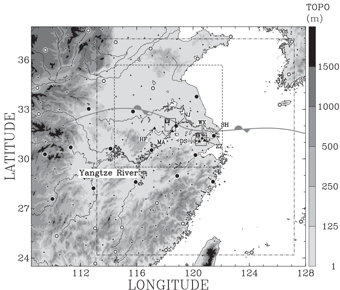
Fig. 1. Geographic map of the Yangtze River. Doppler radar positions (▲), rawinsonde stations (○ for 12-h interval and ● for 6-h interval) and surface stations (+) are shown. Doppler radars are named after the curt names of their locations, with HF being Hefei, MA being Maanshan, DS being Dongshan, WX being Wuxian, ZZ being Zhouzhuang. Boxes with dot-dashed and dashed lines represent the upper-air and surface analysis domains, respectively. The box labeled W indicates the dual-Doppler-radar analysis domain for the HF and MA radars and the box labeled E indicates the triple-Doppler-radar analysis domain for the DS, WX, and ZZ radars. NJ (Nanjing) and SH (Shanghai) indicate the rawinsonde stations where observational data are used to constitute skew-T log p diagrams in Fig. 4. Also shown is the location of the Mei-yu/Baiu front for 0200 LST 21 June 2002.
