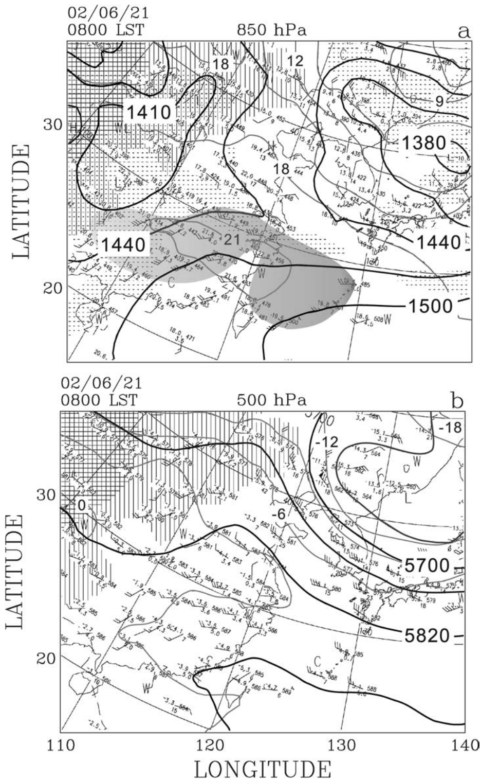
Fig. 3. Synoptic weather maps for 0800 LST 21 June 2002 at (a) 850 hPa, and (b) 500 hPa. Black lines represent geopotential heights (contoured every 50 m) and grey lines represent temperatures (contoured every 3^\circ\text{C} ). Vertical and cross hatches have the same meanings as those in Fig. 2. Dotted regions indicate the areas where the difference between temperature and dew point temperature is less than 3^\circ\text{C} . The shaded region in (a) outlines the area with wind speeds greater than 12 \text{ m s}^{-1} .
