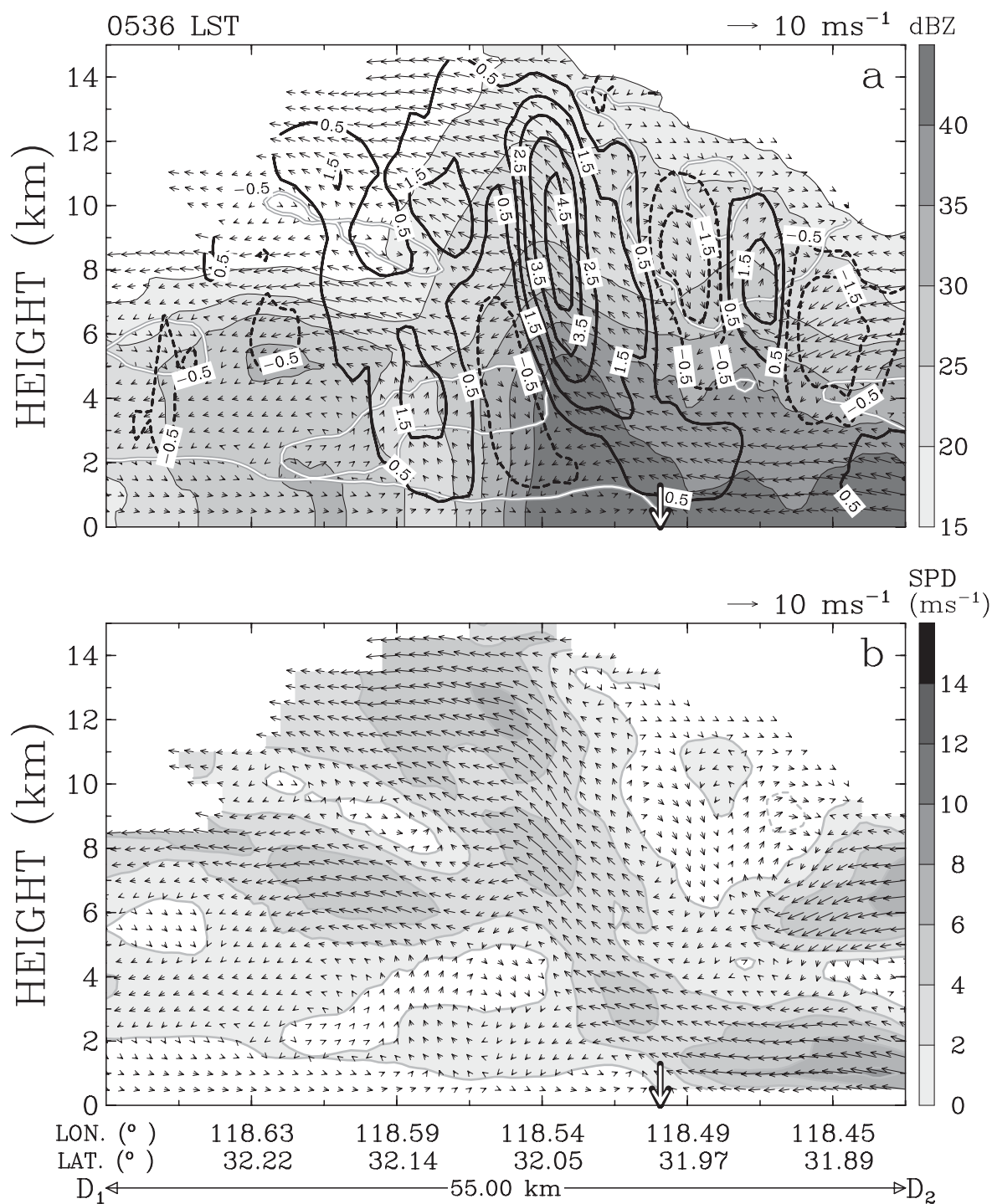
Fig. 13. (a) Vertical cross section of radar reflectivity (shaded), winds along the section plane (arrows), and vertical velocity (contoured every 1 \text{ m s}^{-1} ) for 0536 LST 21 June 2002. The section is along line D_1D_2 in Fig. 11. White solid lines represent interfaces of the positive and negative velocities of horizontal winds along the section plane. The approximate location of the front at the surface is indicated by the white vertical arrow. (b) Same as (a) except for the velocity of the horizontal wind component along the section plane (contoured every 2 \text{ m s}^{-1} and shaded above 0 \text{ m s}^{-1} ).
