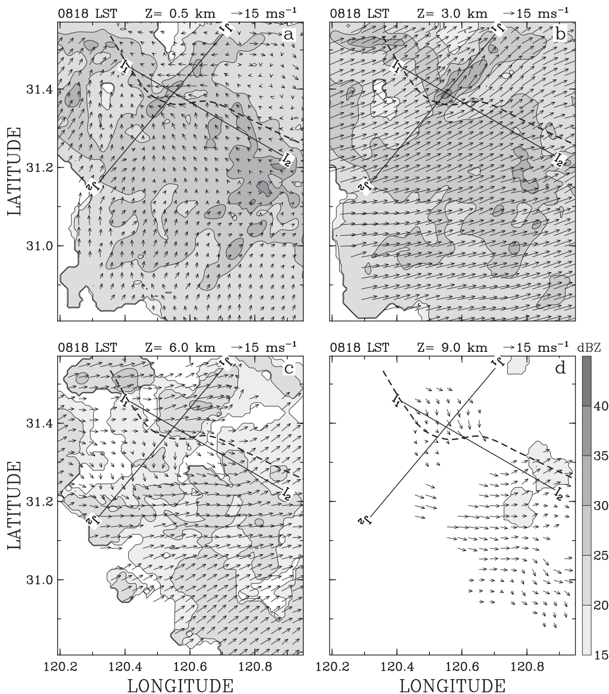
Fig. 20. Same as Fig. 17 except for 0818 LST 21 June 2002. Line I_1I_2 and line J_1J_2 indicate the locations of vertical cross sections shown in Figs. 21 and 22, respectively.
