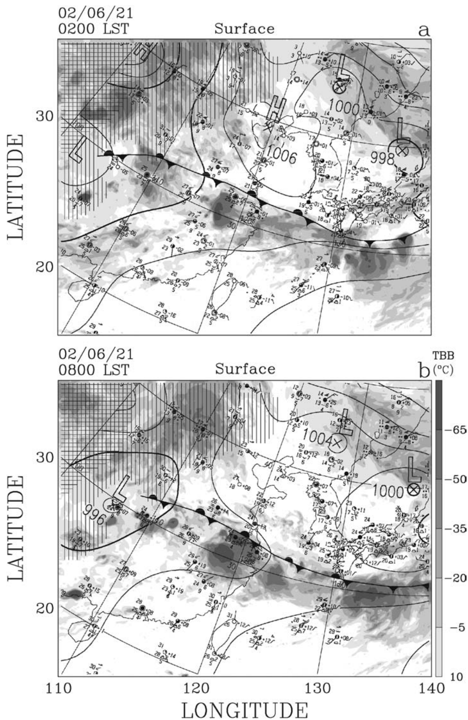
Fig. 2. Surface weather maps superimposed with GMS infrared imageries for (a) 0200 LST, and (b) 0800 LST 21 June 2002. Vertically and crosswise hatched regions represent the areas where topographic altitudes are between 1000 m and 3000 m and higher than 3000 m, respectively.
