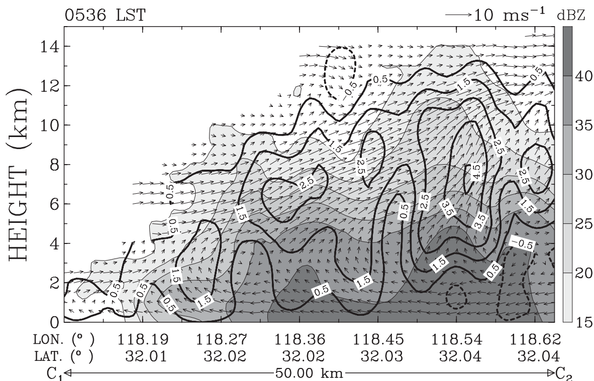
Fig. 12. Vertical cross section of radar reflectivity (shaded), winds along the section plane (arrows), and vertical velocity (contoured every 1 \text{ m s}^{-1} ) for 0536 LST 21 June 2002. The section is along line C_1C_2 in Fig. 11.
