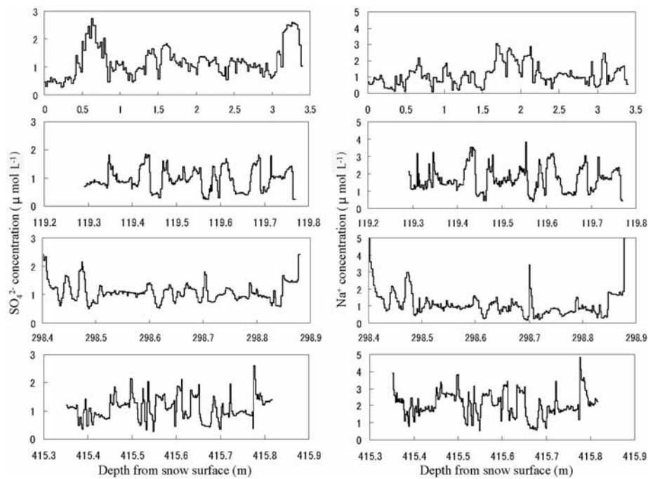
Fig. 2. High-resolution depth profiles of SO 4 2- and Na + concentrations in the surface snow and Holocene ice. Analyses were made in the same manner as described for Figure 1.
