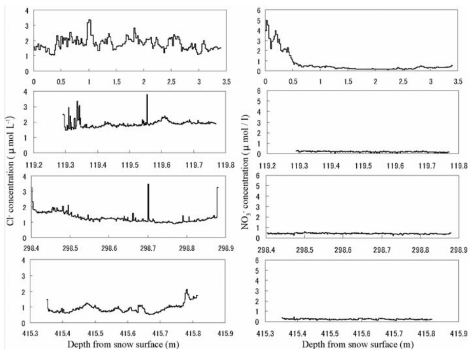
Fig. 1. High-resolution depth profiles of \text{Cl}^- and \text{NO}_3^- concentrations at depths of 0–3.4 m (surface snow), 119, 298 and 415 m. The 119 and 298 m sections are from the Holocene, the 415 m section slightly predates the Holocene but, for simplicity, all three will be called ‘Holocene ice’. Analyses were made every 20 mm of depth for surface snow and every 2 mm of depth for the Holocene ice.
