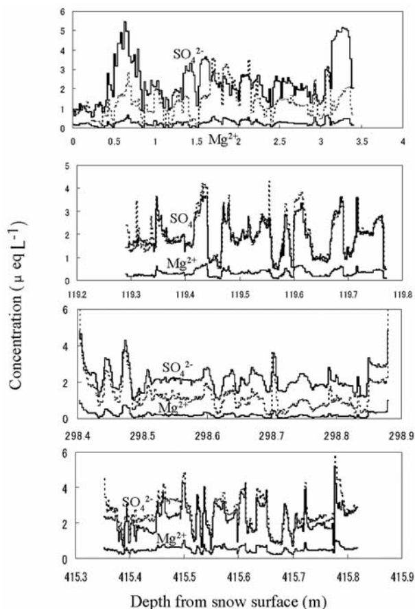
Fig. 3. High-resolution profiles of \text{SO}_4^{2-} , \text{Mg}^{2+} and the sum of \text{Mg}^{2+} and \text{Na}^+ in the surface snow and Holocene ice. The \text{SO}_4^{2-} and \text{Mg}^{2+} profiles are solid black lines and the sum of the \text{Mg}^{2+} and \text{Na}^+ profiles is a dotted line. These concentrations are in equivalent ( \mu\text{eq L}^{-1} ).
