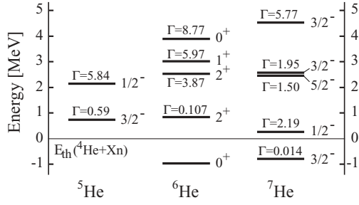
FIG. 4. Energy eigenvalues of the obtained {}^5, {}^6, {}^7\text{He} resonances measured from the {}^4\text{He} + Xn threshold.
