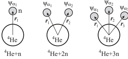
FIG. 2. Sets of the spatial coordinates in the COSM for the {}^4\text{He} + Xn system.
