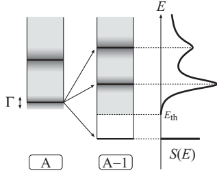
FIG. 1. Schematic illustration of the one-nucleon removal strength S(E) , from the mass A system to the A - 1 one. The excitation energy E is for the A - 1 system. E_{th} is the lowest threshold energy of particle emission for the A - 1 system.
