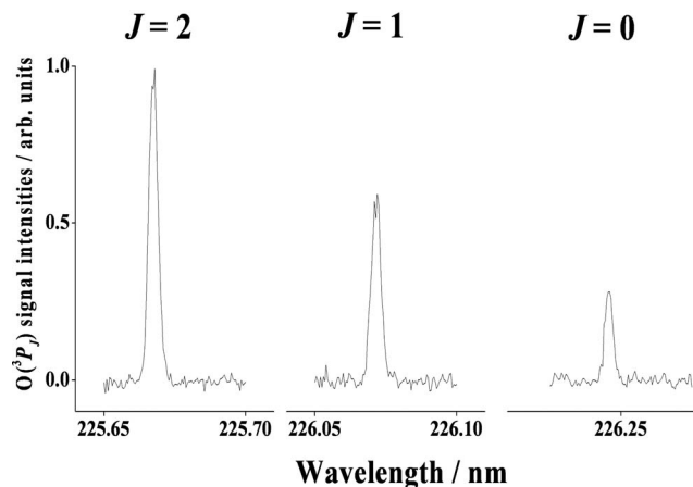
FIG. 1. REMPI excitation spectra of the O(^3P_J \leftarrow ^3P_J) transition from the 157 nm photodissociation of fresh ASW at 90 K. TOF = 2.5 \mu\text{s} .
