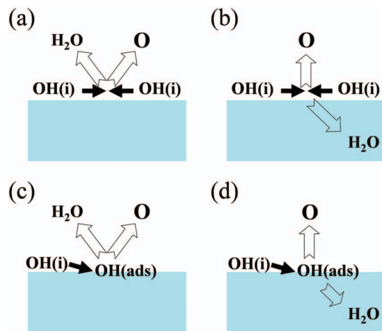
FIG. 5. Schematic illustrations of the collisional recombination reactions of OH radicals on the surface of ice for forming O(^3P_j) atom, (a) reaction (13), (b) reaction (14), (c) reaction (15), and (d) reaction (16). OH(i) stands for OH radical at the ASW/vacuum interface, and OH(ads) stands for adsorbed species.
