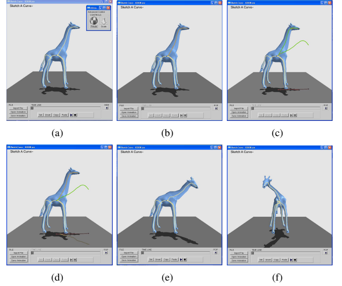
Fig. 2. (a) The user can easily rotate or scale the 3D model by a pop-up window. (b) Initially, a target skeleton is selected. (c) The user draws a new skeleton curve on the view plane. (d) The user can draw another curve for z-axis through its projected skeleton in shadow on the ground plane. (e) and (f) Two different views of the editing result.
