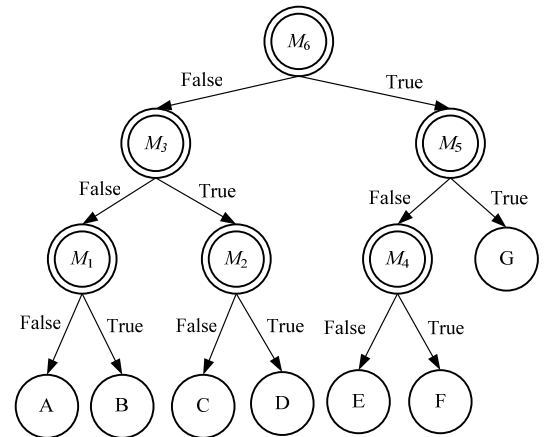
Fig. 12 An example of a multi-classifier for discriminating seven classes.
