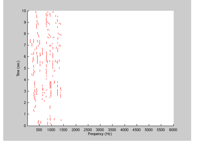
Fig. 4. Vocal sinusoids extracted from a 10-second song clip. Here in adaptive Wiener filtering, the signal is represented by power spectra bandlimited to 1.4 kHz, and modulated sinusoids distributed above that frequency are unconditionally excluded from this collection of vocal sinusoids.
