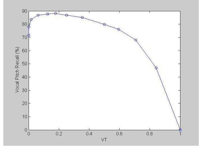
Fig. 9. Vocal pitch recalls with various vocalicity thresholds. NB = 129; FC = 1.4 kHz; KV = 32; KA = 1024.
