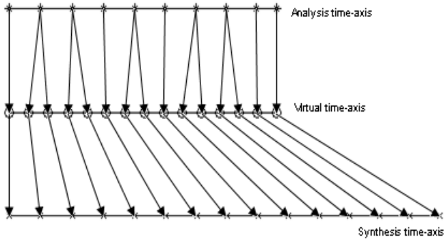
Fig. 2. Estimation of Synthesis Time-instants for Diphone /a-a/
