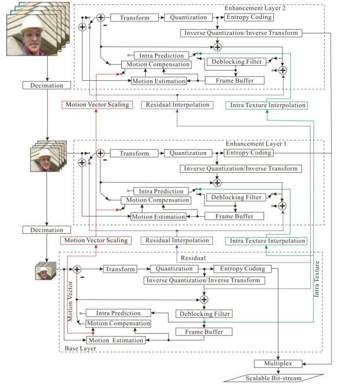
Fig. 1 Spatial scalability architecture of SVC
