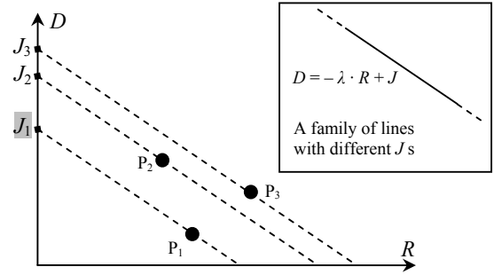
Fig. 1. Visualizing the Kernel Selection Process
