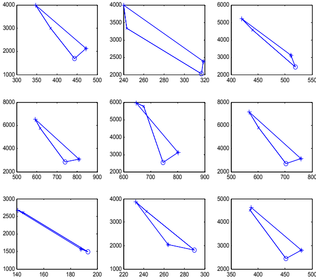
Fig. 5. Nine MLKGs (out of a total of 393 MLKGs) of the I-Frame of Sequence Tempete at QP = 24 .
