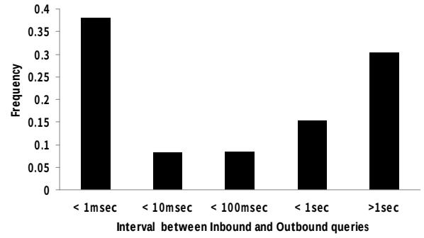
Figure.5 Distribution of time spent for routing and forwarding a query message by Winnie
