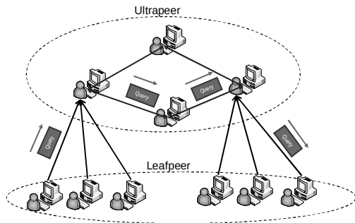
Figure.2 Topology of LimeWire Network
