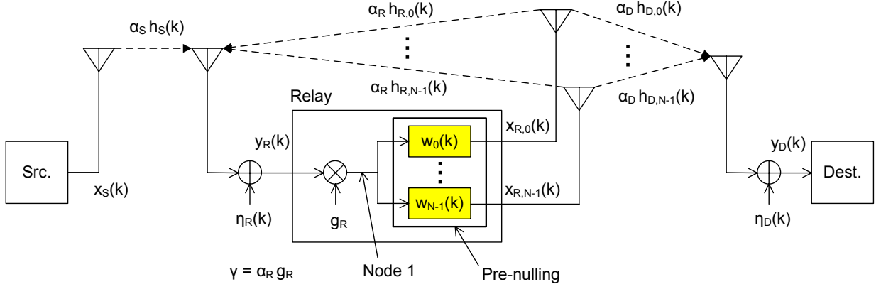
Fig. 1. A full-duplex AF relay system employing the proposed pre-nulling filters for interference suppression at the relay.
