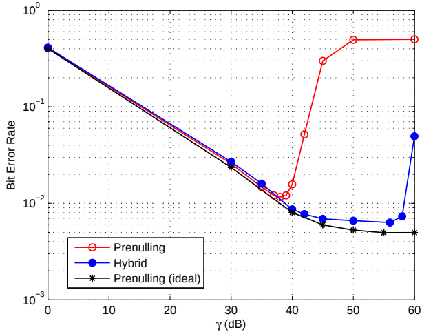
Fig. 6. BER performance at the destination versus \gamma when pre-nulling and hybrid methods are used at the relay, respectively. \sigma_e^2 = 10^{-5} assumed for both cases, but \sigma_e^2 = 0 for ideal pre-nulling. Flat Rayleigh fading, uncoded BPSK modulation, and matched filter bound are assumed.
