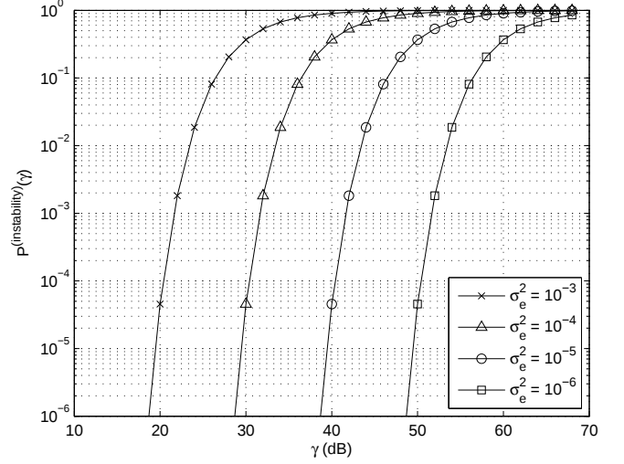
Fig. 2. Theoretically calculated probabilities of instability as a function of \gamma in the flat interference channel for the channel estimation error variances \sigma_e^2 = 10^{-3}, 10^{-4}, 10^{-5}, 10^{-6} , respectively.
