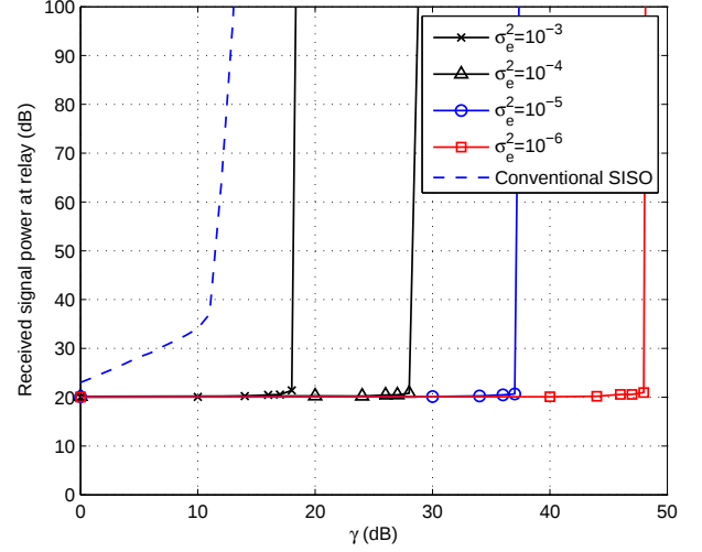
Fig. 4. Received signal power at the relay versus \gamma for \sigma_e^2 = 10^{-3}, 10^{-4}, 10^{-5}, 10^{-6} , respectively. Note that, in the case of the conventional SISO, the received signal power at the relay increases with an apparent slope as \gamma increases due to addition of the interference whereas those for the proposed scheme do not exhibit such phenomena until reaching the critical points thanks to the pre-nulling. Also, note that the critical points almost coincide with those where P(\text{instability}) = 10^{-6} in Fig. 2. This can be easily understood since even single event of oscillation out of 10^6 independent trials for given \gamma will cause the plot to diverge at the \gamma value.
