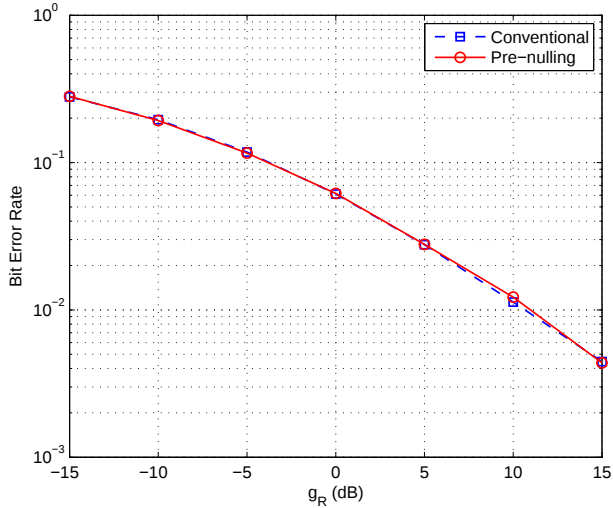
Fig. 7. BER performance at the destination as a function of g_R according to the conventional SISO method and the proposed pre-nulling method. Flat Rayleigh fading, uncoded BPSK modulation, and matched filter bound are assumed.
