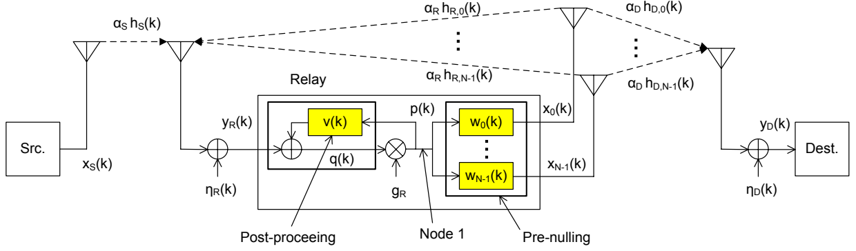
Fig. 3. A full-duplex AF relay system employing the hybrid method for interference suppression at the relay.
