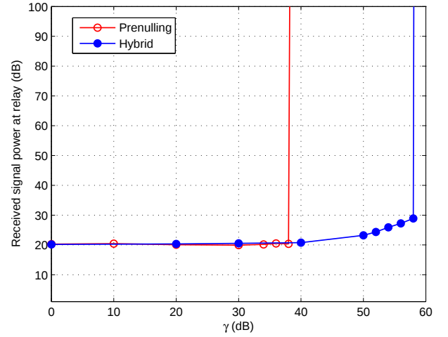
Fig. 5. Received signal power at the relay versus \gamma according to the pre-nulling and hybrid methods. \sigma_e^2 = 10^{-5} assumed.
