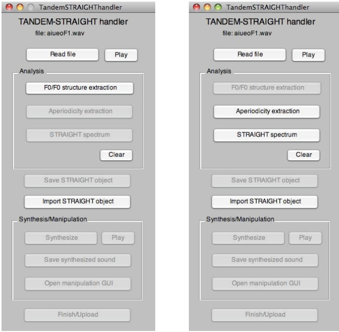
Fig. 4. Left: Initial state of the STRAIGHT handling menu. Right: State after F0 extraction. Note that only buttons that invoke relevant functions are highlighted and the sound file name under analysis is displayed just under the title.
