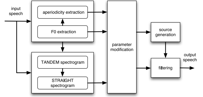
Fig. 1. Schematic diagram of TANDEM-STRAIGHT. Manipulation block modifies source parameters (F0 and aperiodicity) and STRAIGHT spectrogram as well as their coordinates (time and frequency axes).
