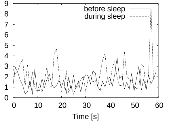
Fig. 3. Power spectrum of the theta component.
