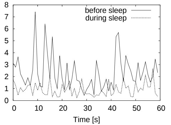
Fig. 4. Power spectrum of the alpha component.
