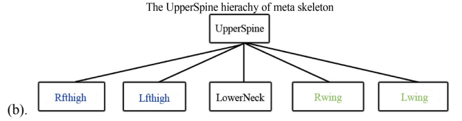
Figure 5: (a) Hierarchy C^{S_b} (b) Loading the skeleton C_1^s (c) Loading the skeleton C_2^s
