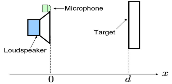
Fig. 1. Positions of loudspeaker, microphone and target.
