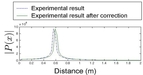
Fig. 8. Range spectra in simulation with single target.
