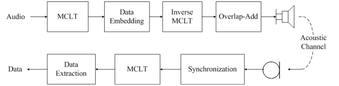
Fig. 1. The proposed acoustic data transmission system.
