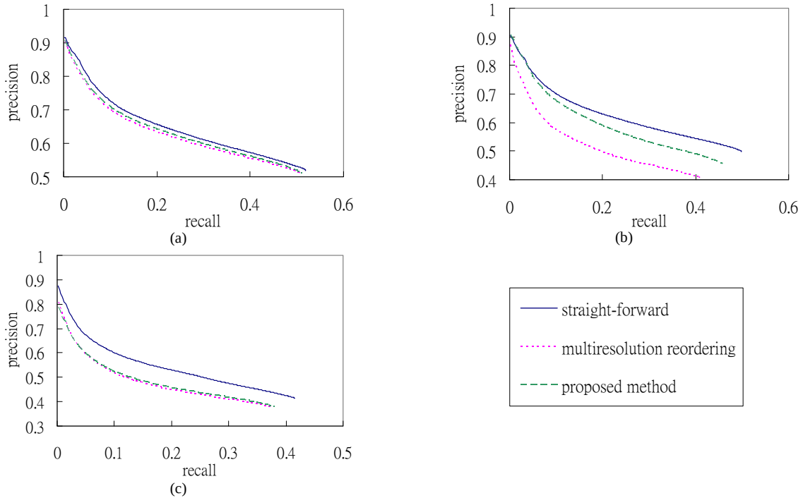
Figure 2. Average precision vs average recall at compression ratio (a) 1.6, (b) 10 and (c) 40.
