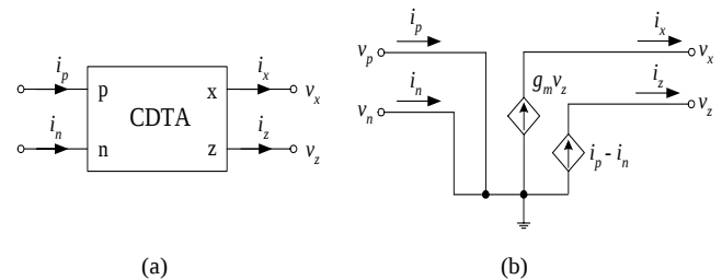
Fig. 1 : CDTA (a) circuit symbol (b) equivalent circuit
