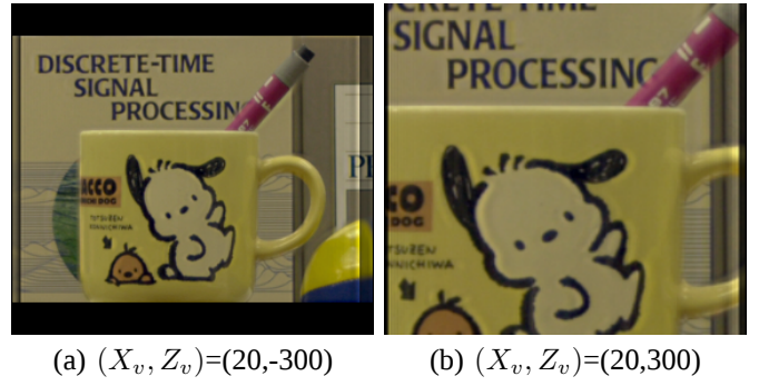
Fig. 8. Example of the novel views synthesized by LFR from the densely interpolated images. (X_v, Z_v) are the coordinates of the novel viewpoint along the horizontal and depth axes.
