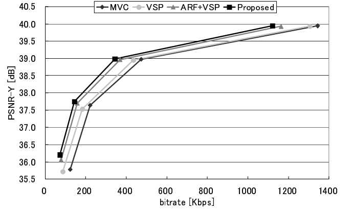
Fig. 2. Overall RD performance
