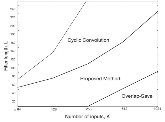
Fig. 4. Effective regions for each filtering methods
