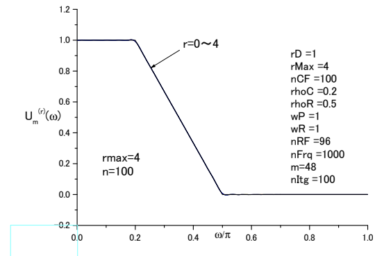
Fig.9 U_m^{(r)}(\omega) for n=100
