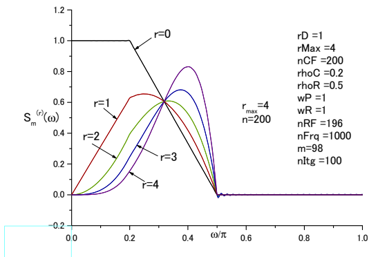
Fig.11 S_m^{(r)}(\omega) for n=200
