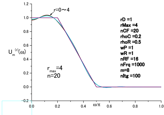
Fig.6 U_m^{(r)}(\omega) for n=20
