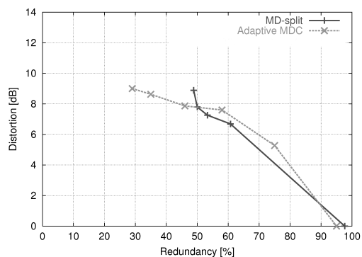
Fig. 2. RRD curves for three video clips (football)
