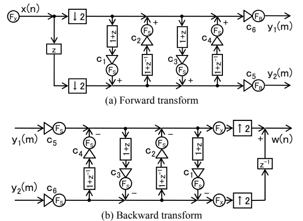
Fig.1 Irreversible 9-7 DWT.
