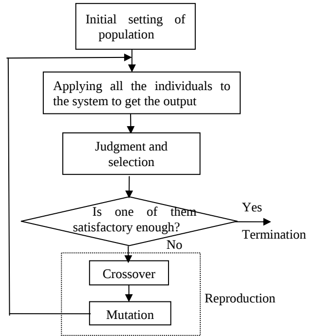
Fig.2 The procedure of the genetic algorithm
