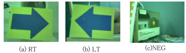
Fig. 8 Training Samples(1)
