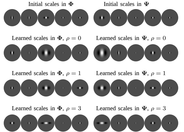
Fig. 2. Subset of atoms in the initial and learned dictionaries for the left and right images. All atoms are on the North pole.
