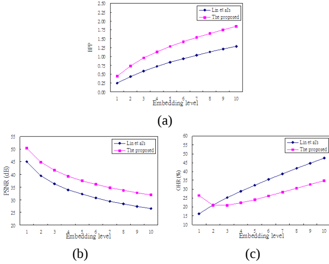
Fig. 5. The average hiding performance comparisons at various embedding levels between the two concerned algorithms. (a) BPP comparison. (b) PSNR comparison. (c) OHR comparison.
