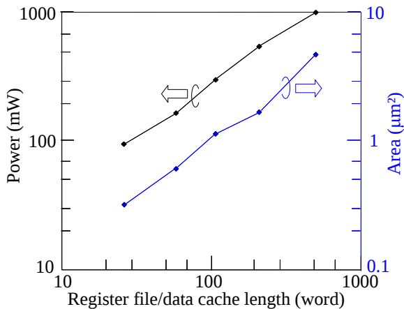
Fig. 6 Power vs. register file length.
