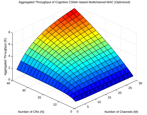
Fig. 5. Aggregated multichannel throughput with p = p^*
