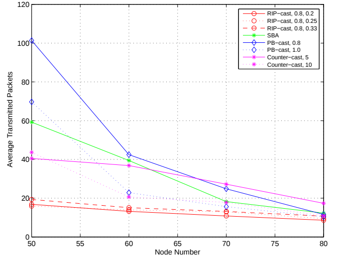
Fig. 7. The average transmitted packets versus the number of nodes in the network.
