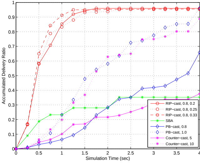
Fig. 6. The accumulated delivery ratio along the simulation time for a network consisting of 80 nodes.
