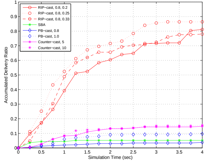
Fig. 3. The accumulated delivery ratio along the simulation time for a network consisting of 50 nodes.
