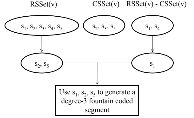
Fig. 2. An Example of the segment selection.
