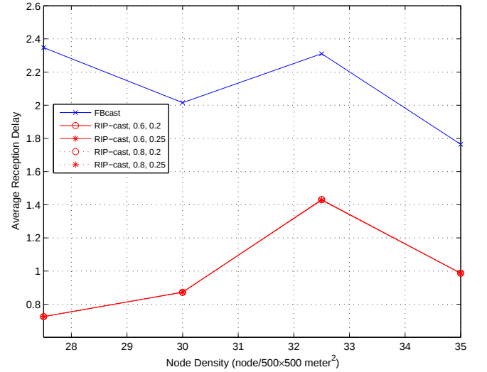
Fig. 8. The average reception delay versus the node density.
