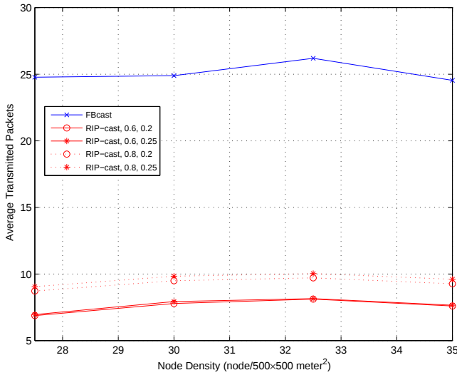
Fig. 9. The average transmitted packets versus the node density.
