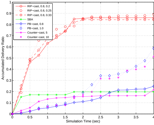
Fig. 5. The accumulated delivery ratio along the simulation time for a network consisting of 70 nodes.
