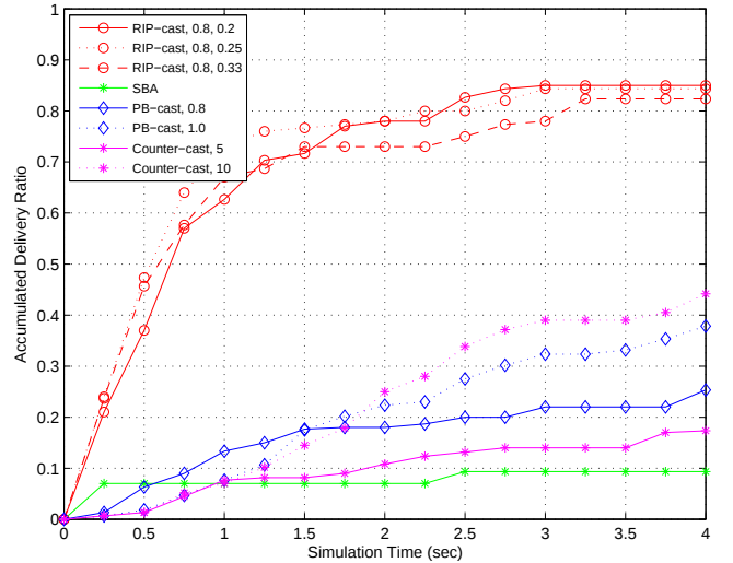
Fig. 4. The accumulated delivery ratio along the simulation time for a network consisting of 60 nodes.
