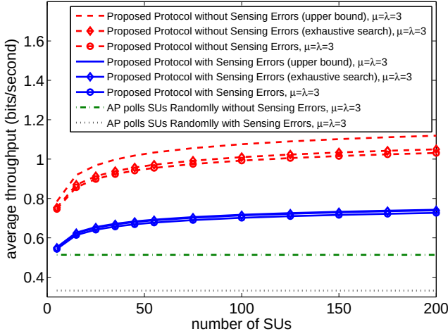
Fig. 8. Network throughput versus the number of SUs with K = 6 .
