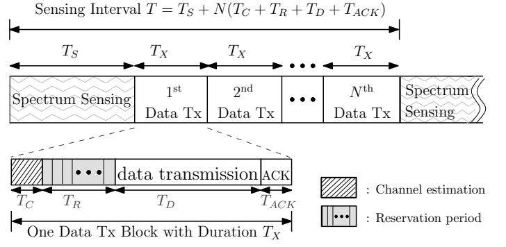
Fig. 3. Time slot model.
