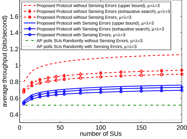
Fig. 7. Network throughput versus the number of SUs with K = 4 .
