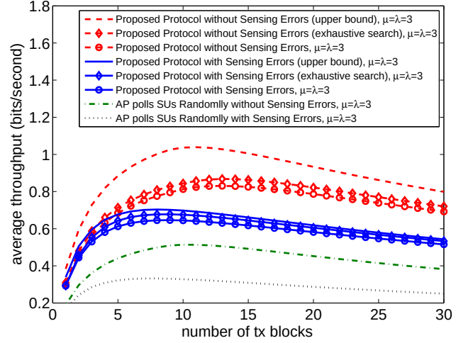
Fig. 6. Network throughput versus the number of transmission blocks.
