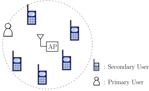
Fig. 1. Network model.
