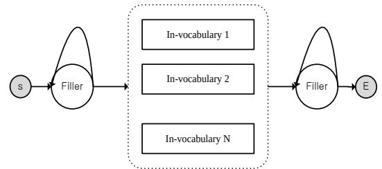
Fig. 1: A typical finite state network for one-keyword spotting.
