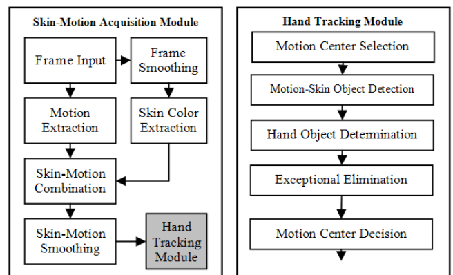
Fig. 1 The block diagram of hand tracking
