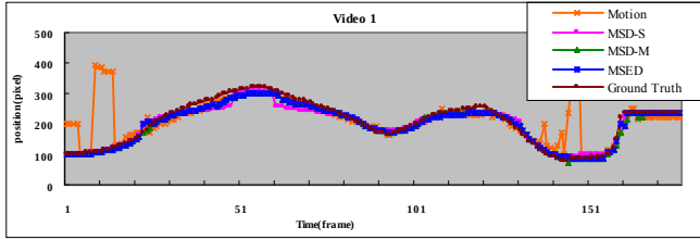
Fig. 6 The results of each steps in our method for video 1.
