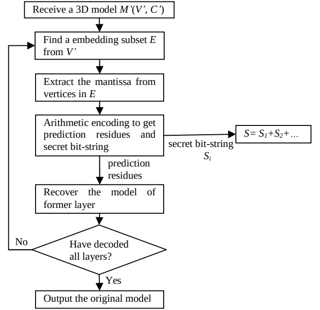
Fig. 4 Overview of the decoding scheme
