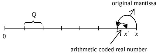
Fig. 3 The mantissa substitution scheme
