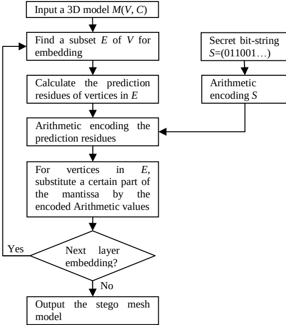
Fig. 1 Overview of the embedding scheme
