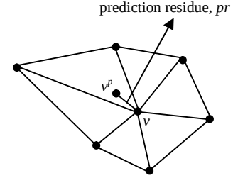
Fig. 2 The prediction residue v is the vertex for embedding v^p is predicted by v 's surrounding vertices.
