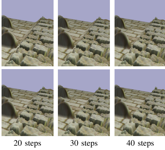
Fig. 4 Comparisons of convergence between CSM and ACM. The top row shows convergence of CSM and the bottom row is for ACM. Note that, on the discontinuity border in the middle, CSM at 20 steps appears too flat. However, ACM at 20 steps is already very close to the final solution.
