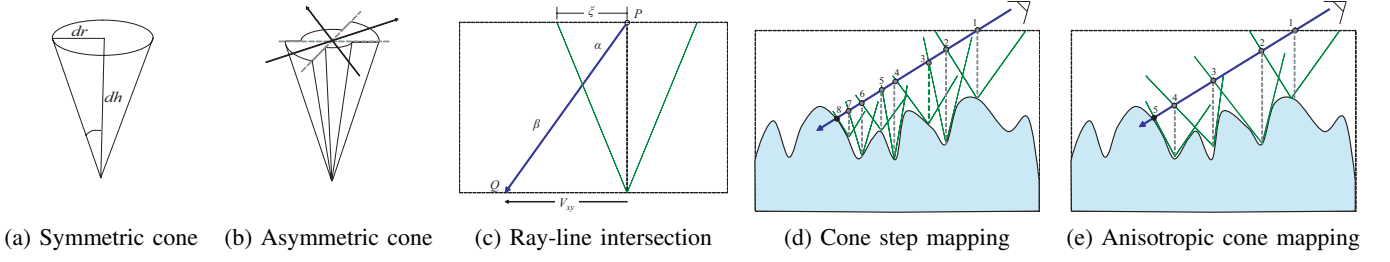
Fig. 1 Configuration of symmetric (a) and asymmetric cones (b). (c) illustrates our ray-line intersection algorithm. (d) and (e) show how CSM and ACM work.
