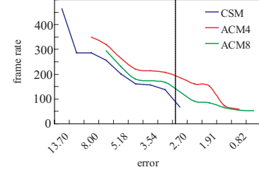
Fig. 3 Comparisons of error and frame rate among CSM, ACM4 (4-sector ACM) and ACM8 (8-sector ACM).
