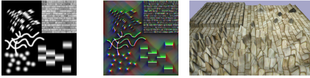
(a) Displacement map (b) ACM texture (c) Rendering
