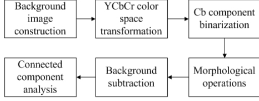
Fig. 1: Block diagram of pre-processing.
