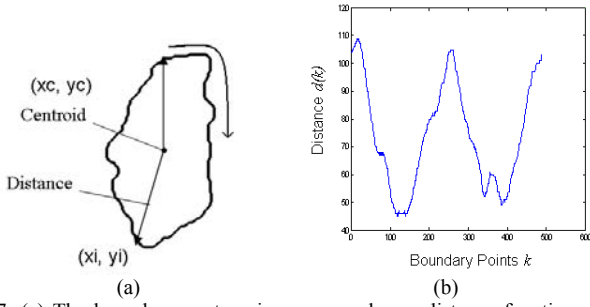
Fig. 7: (a) The boundary contour is unwrapped as a distance function with respect to the centroid. (b) The one-dimensional waveform signal representing the distance between the centroid and the edge points in (a).
