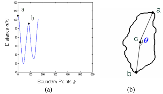
Fig. 11: (a) Two peak points in the waveform. (b) The angle \theta between the two peak points and the centroid.
