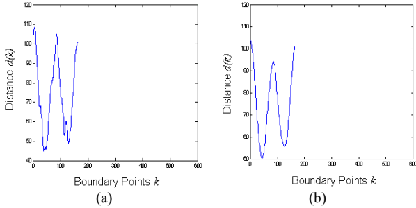
Fig. 8: (a) Sub-sampled result of waveform. (b) Smoothed result of waveform.
