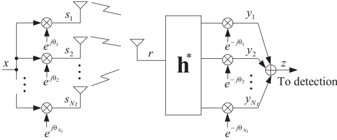
Fig. 1. A block diagram of the equal gain precoder.
