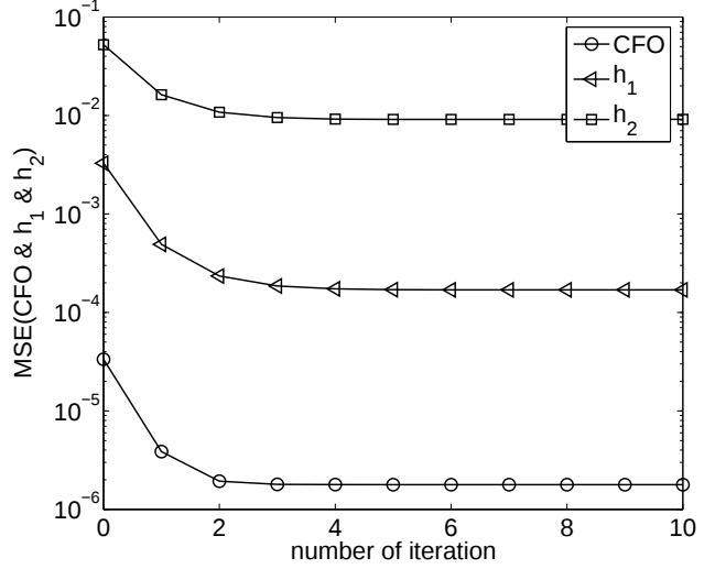
Fig. 2. MSE vs. iteration number
