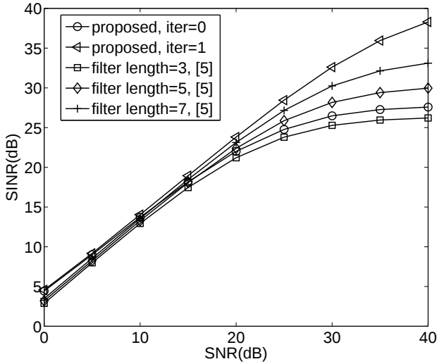
Fig. 4. SINR performance
