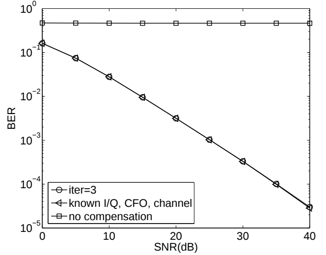
Fig. 5. BER performance
